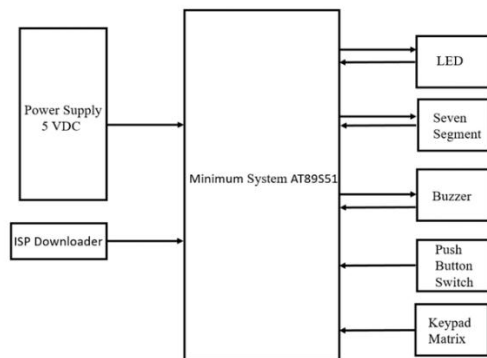
Gambar 3.1 Blok Diagram Basic Operation Trainer AT89S51
